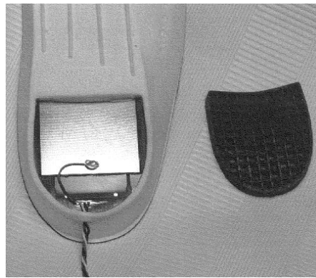
Figure 8: PZT generator embedded in an insole. Power is generated by the user's heel striking (and flattening) the PZT clamshell.
